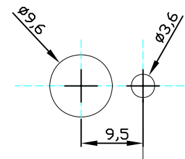
Shaft end installation size
